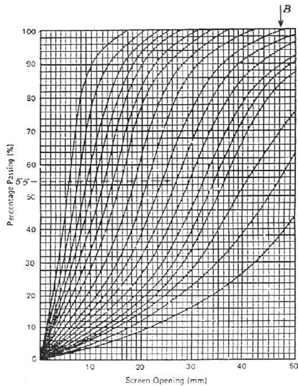
Gambar 6 - Cone Crusher Analysis (Product Gradation Curve)
